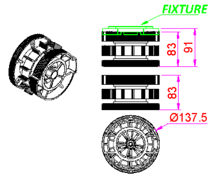
Adjustable feet, Lowest Height 91mm
