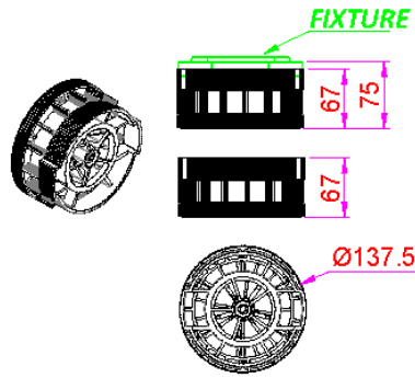
Adjustable feet, Lowest Height 75mm
